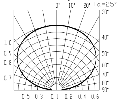
Radiation Diagram
